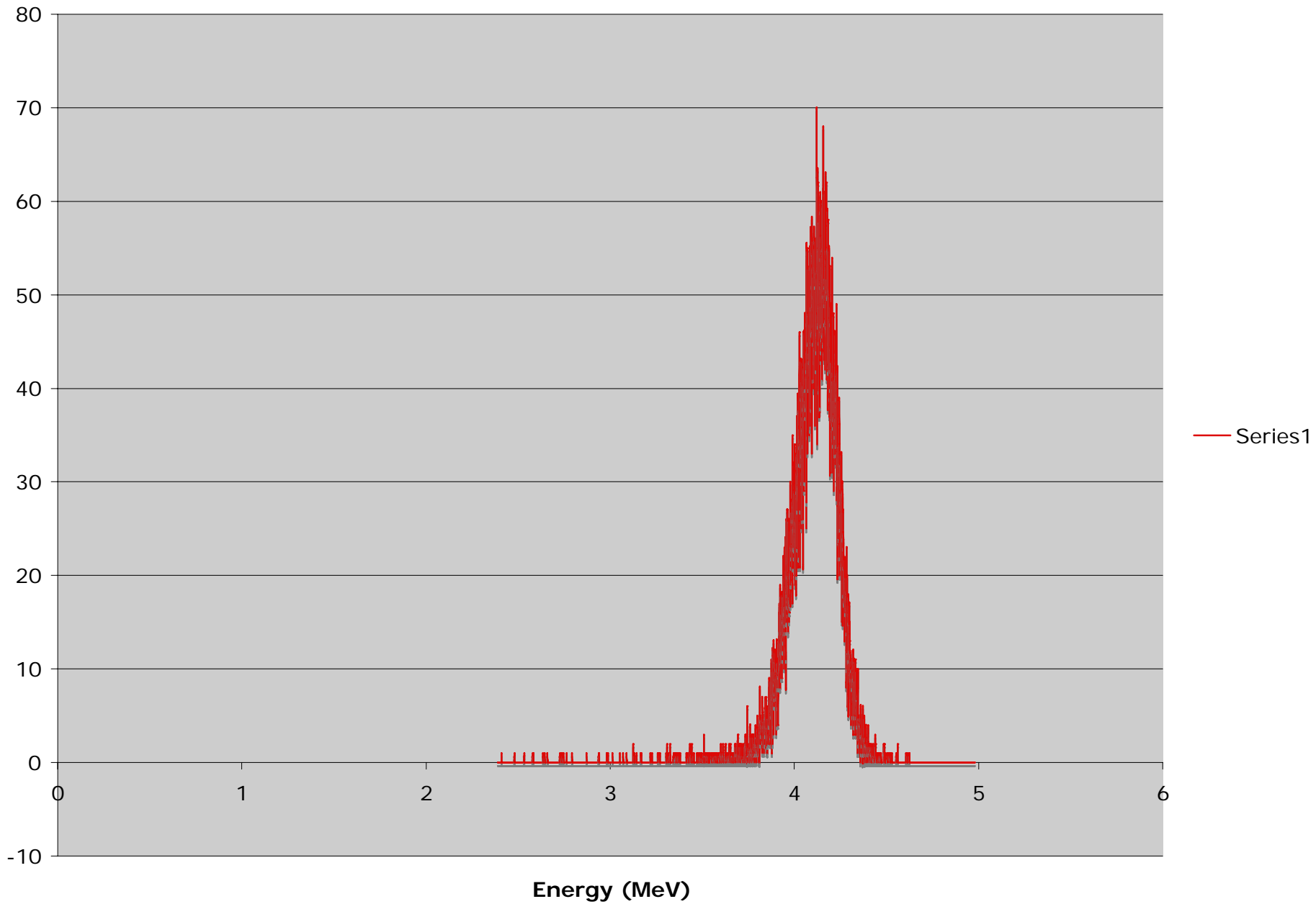
Am241- Aluminum foil: Counts vs. Energy
