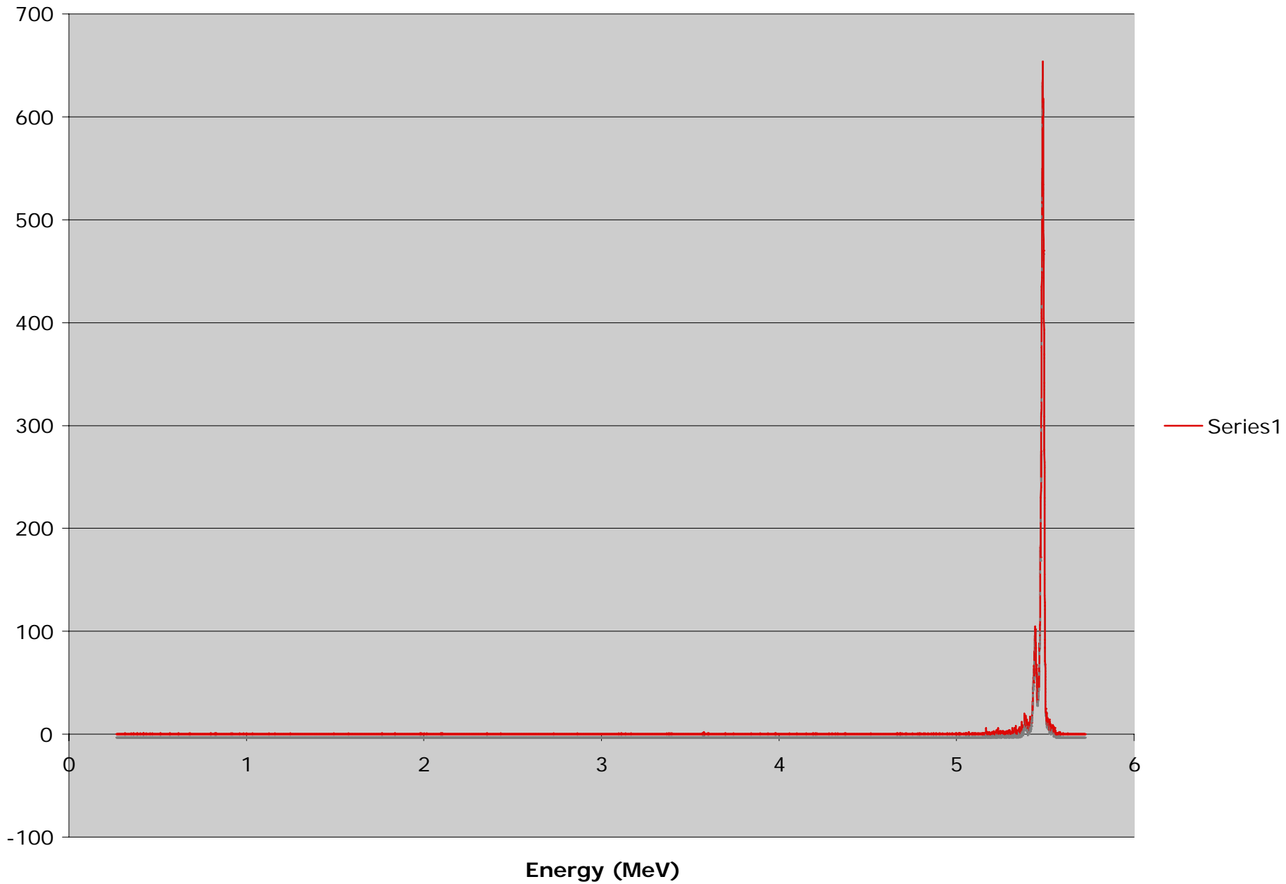
Am241- no foil: Counts vs. Energy
