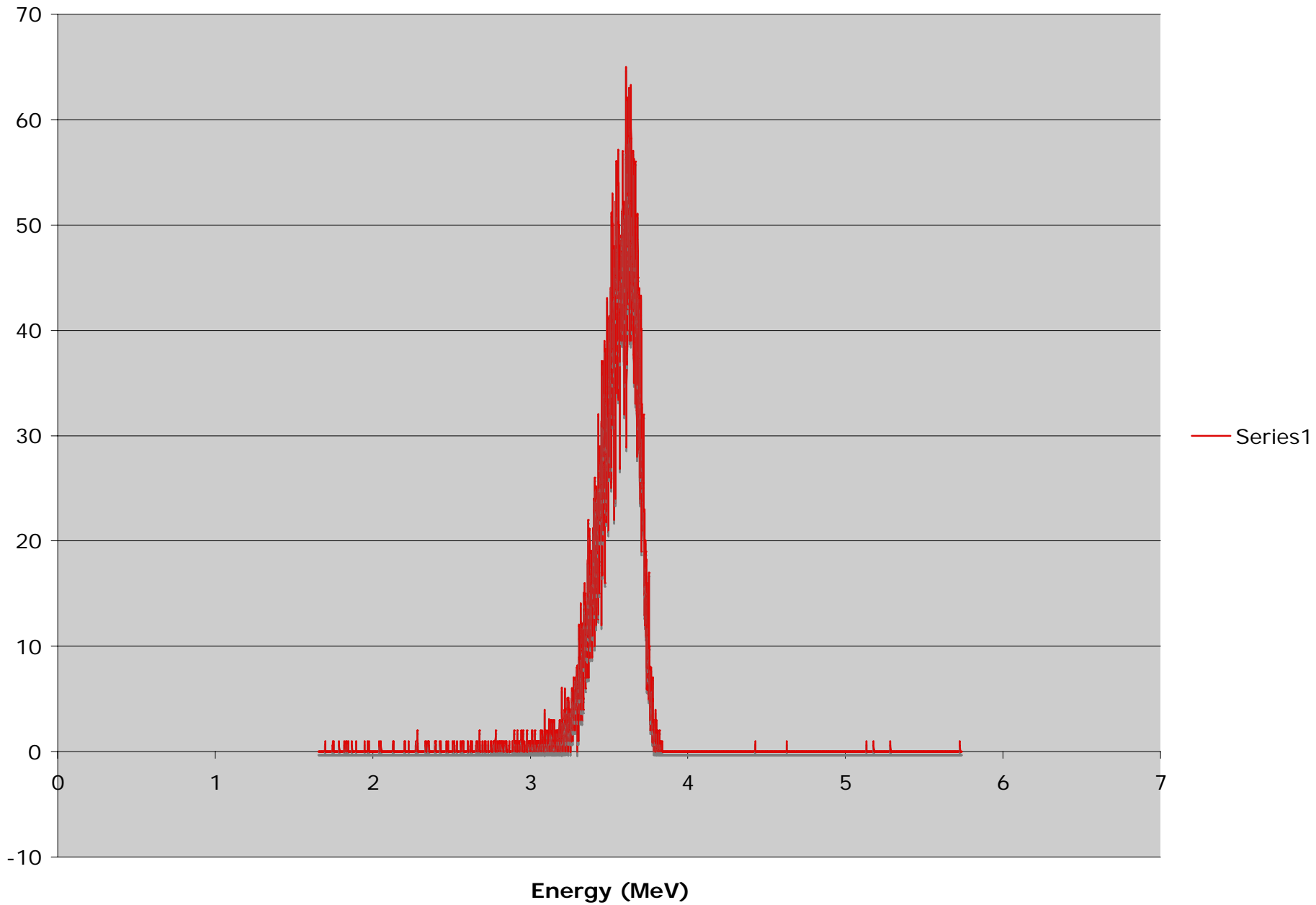
Am241- Havar foil 4.6 um: Counts vs. Energy
