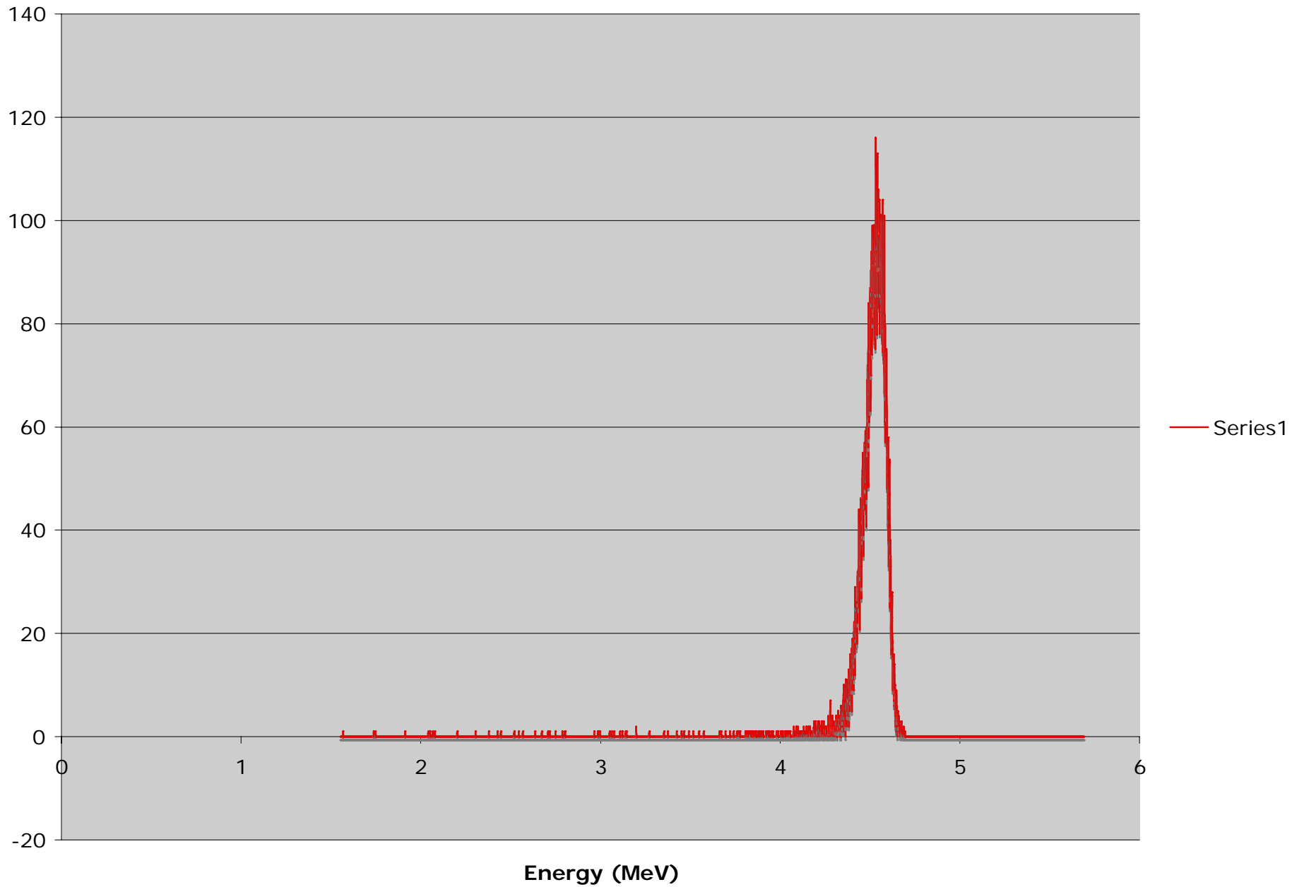
Am241- Havar foil: Counts vs. Energy
