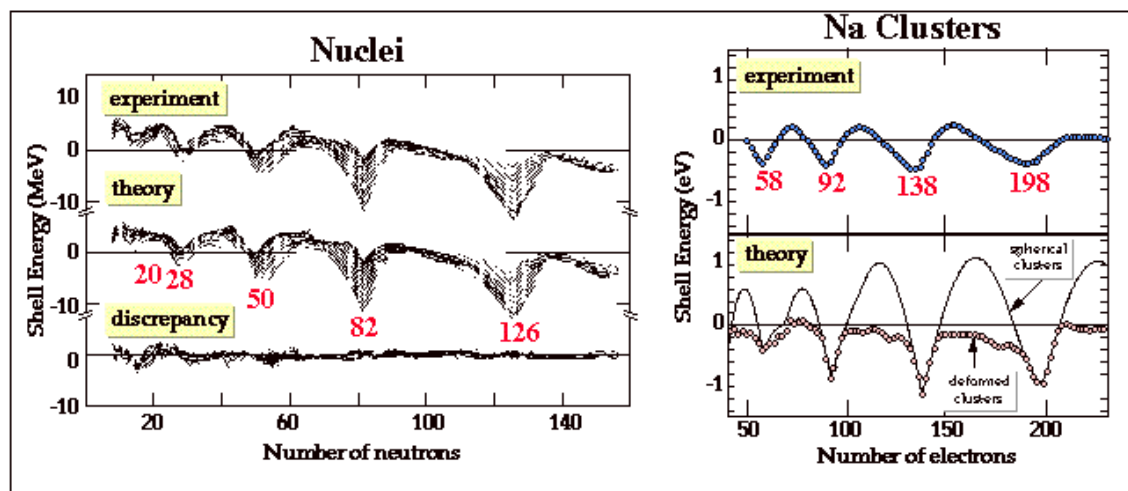
Fig. 1. Experimental and calculated shell energies for nuclei (left) and sodium clusters (right) as a function of particle number (neutrons for nuclei and electrons for clusters). The sharp minima can be attributed to the presence of magic gaps.
