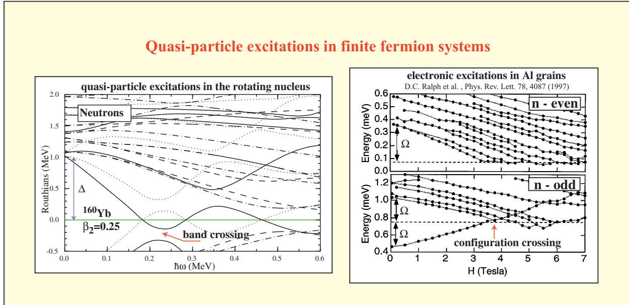
Fig. 2. Quasi-particle excitations in femto-and nano-structures. Left: Quasi-particle neutron spectrum of rotating ^{160}\text{Yb} as a function of rotational frequency \hbar\omega calculated assuming neutron pairing gap \Delta_n=1 MeV and quadrupole shape deformation \beta=0.25 . Right: Measured electronic excitations in Al grains as functions of the external magnetic field.
