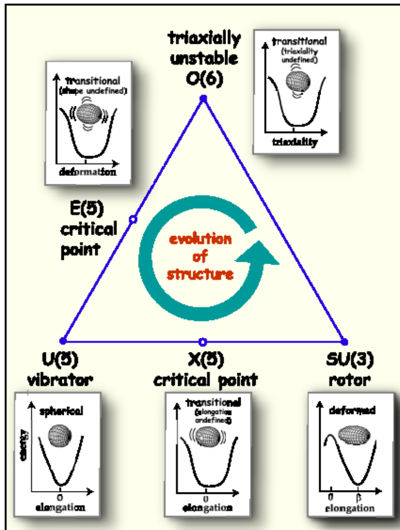
Fig. 4. Symmetry triangle for collective manifestations of nuclear structure showing the dynamical symmetries of the Interacting Boson Model at the vertices and critical point symmetries on the legs. The inserts show the nuclear energy surface as a function of appropriate shape parameters.
