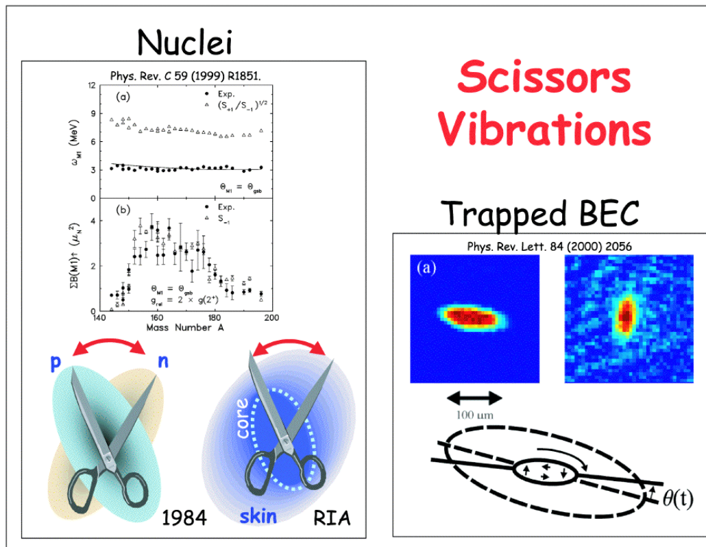
Fig. 3. Scissors modes in deformed superfluid nuclei (left), showing some of the energy and transition rate data supporting the concept, and a similar depiction of trapped Bose-Einstein condensate of {}^{87}\text{Rb} atoms (right).
